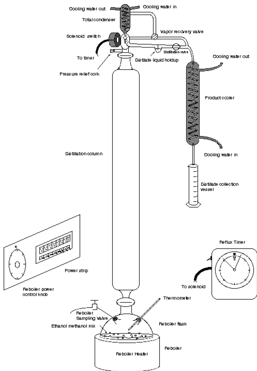
Figure 1. Experimental Apparatus for Batch Distillation
